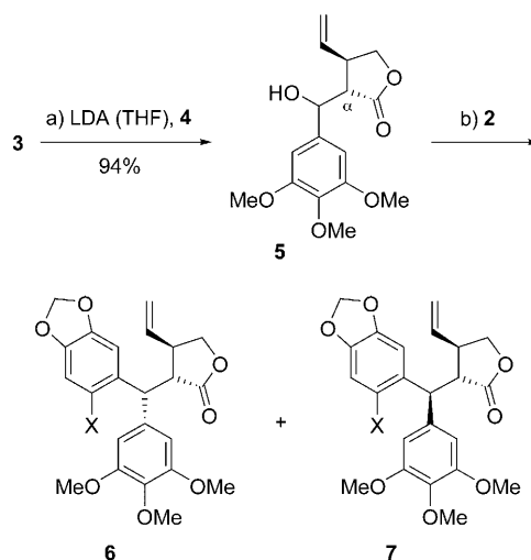
Scheme 2. Aldol reaction and subsequent intermolecular Friedel–Crafts alkylation: a) LDA (1.1 equiv), THF, –78 °C, 30 min, then 4 (1.1 equiv), –78 °C, 3 h, 94% (d.r. 52:48); b) see Table 1. LDA = lithium diisopropylamide.
