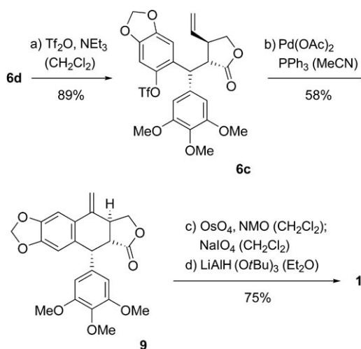
Scheme 4. Completion of the total synthesis of (–)-podophyllotoxin ( 1 ): a) Tf 2 O (1.5 equiv), NEt 3 (2 equiv), CH 2 Cl 2 , 0 °C, 1 h, 89%; b) Pd(OAc) 2 (10 mol %), PPh 3 (0.3 equiv), K 2 CO 3 (3 equiv), MeCN, 80 °C, 20 h, 58%; c) OsO 4 (5 mol %), NMO (3 equiv), CH 2 Cl 2 , 20 °C, 4 h, then NaIO 4 (2 equiv), 30 min, 95%; d) LiAlH (OtBu) 3 (10 equiv), Et 2 O, –78 → 20 °C, 18 h, 79% (d.r. 98:2). Tf = trifluoromethanesulfonyl.
